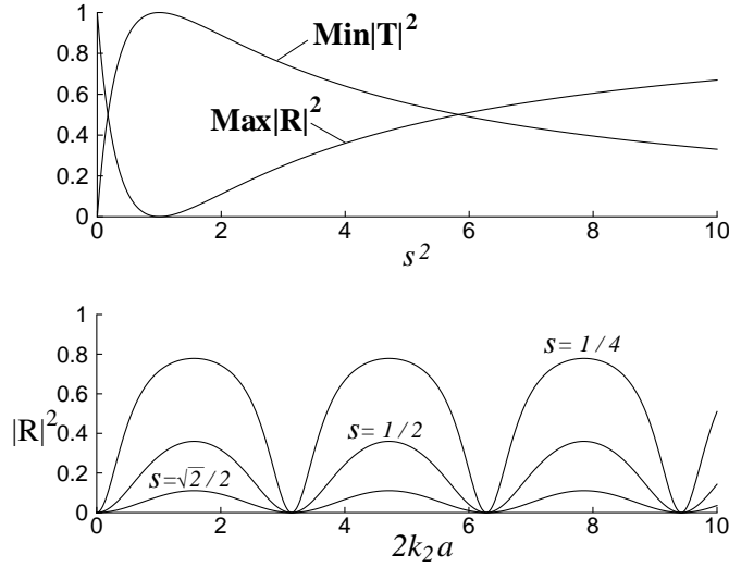
Figure 7: Transmission and reflection coefficients for a rectangular shelf. From Mei, C.C., Applied Dynamics of Ocean Surface Waves .
